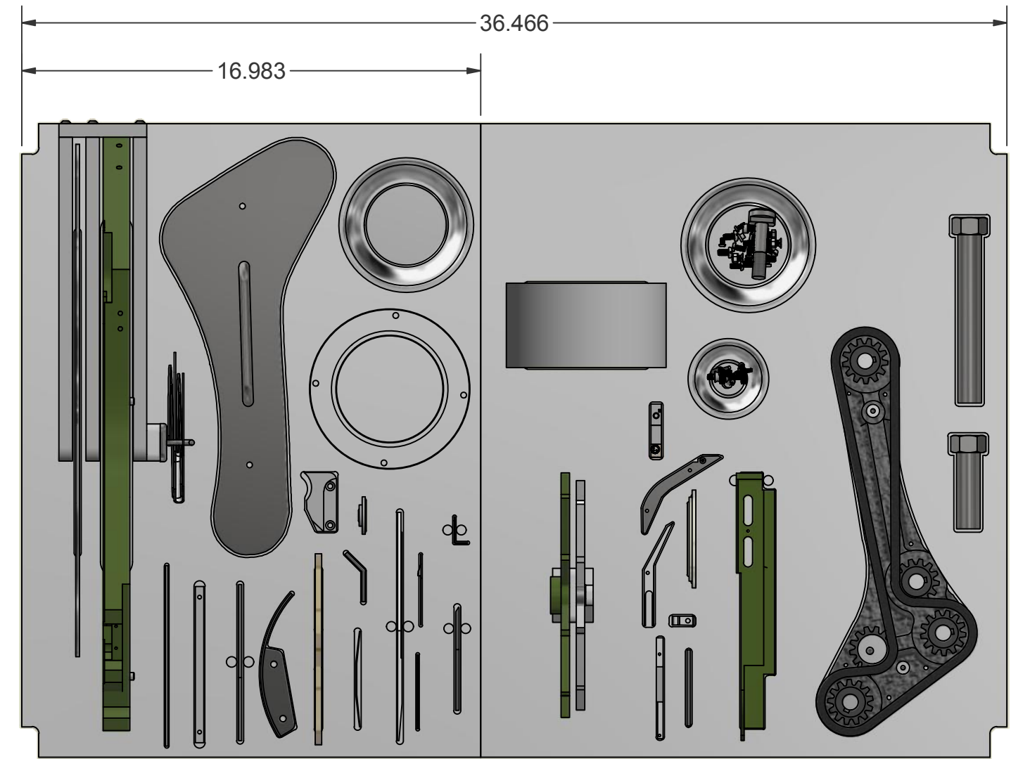
NOVA-00-102 ADJUSTABLE SHELF, FEEDER COMPONENTS ASSY SCALE .2
