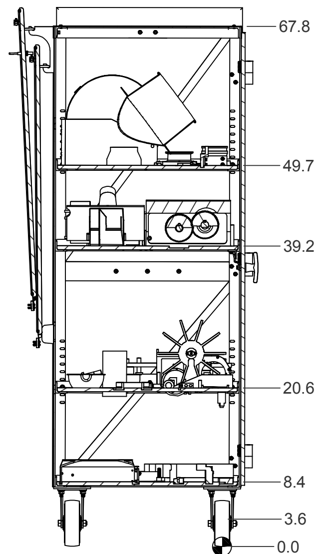
SECTION A-A SHELF HEIGHT SCALE 0.08 : 1
