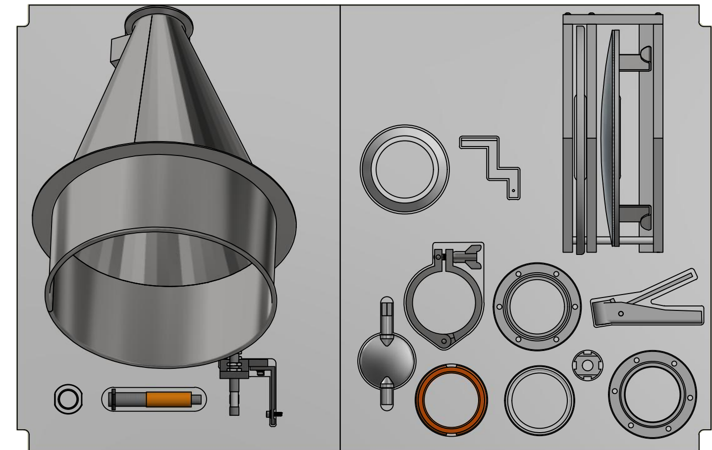
NOVA-00-103 ADJUSTABLE SHELF, HOPPER COMPONENTS ASSY SCALE .2
