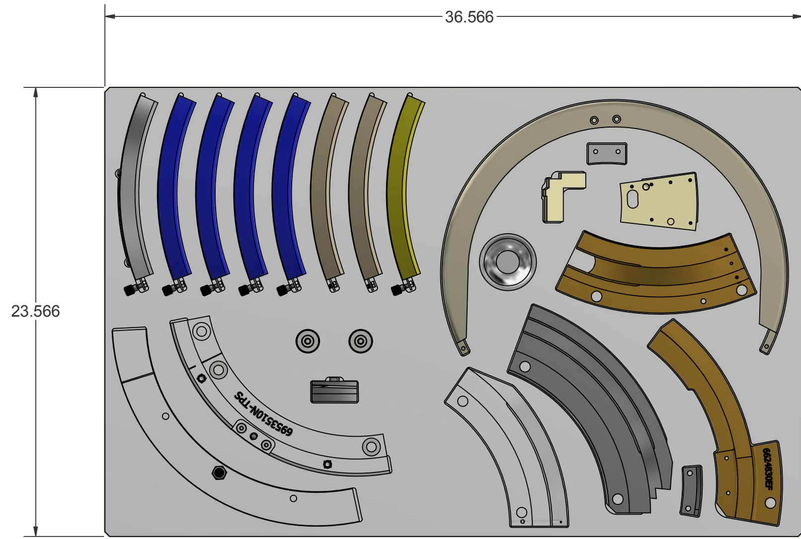
NOVA-00-100 SHELF, CAM COMPONENTS ASSY SCALE .2
