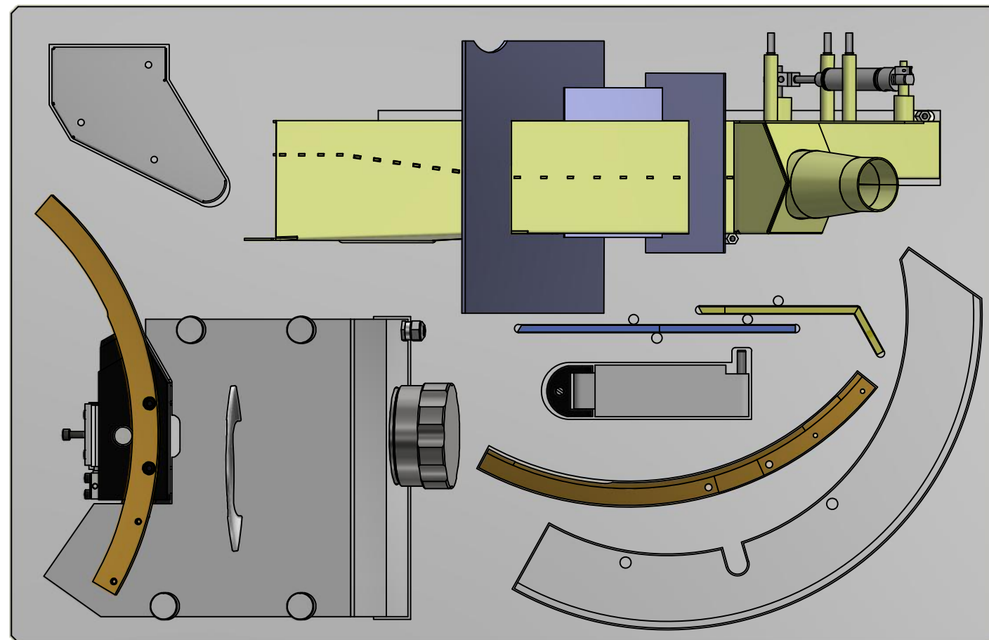
NOVA-00-101 SHELF, WEIGHT & CHUTE ASSY SCALE .2
